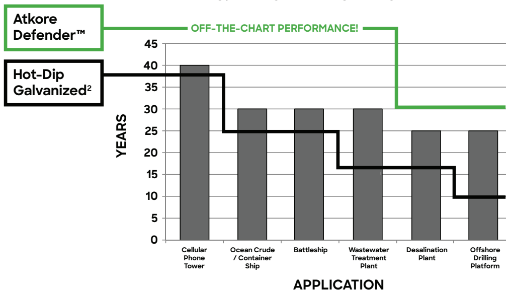
TYPICAL APPLICATION DESIGN LIFE 1 VS. ANTICIPATED SERVICE LIFE
