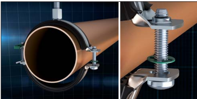
Distance ring for easy installation
