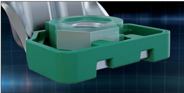
Hammer with captive nut
