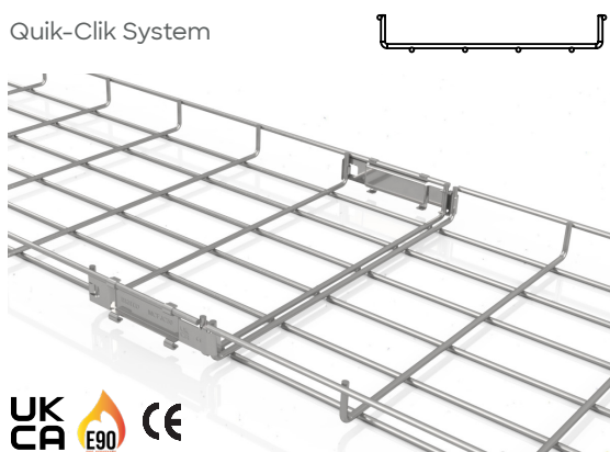
Quik-Clik System
