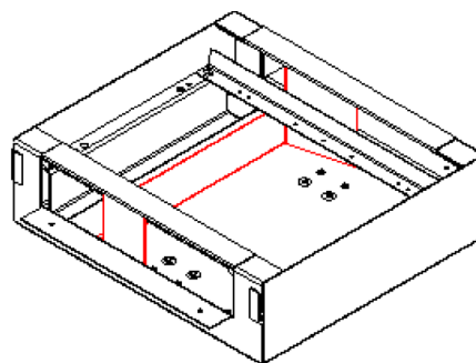
4/2OC* - 4 Compartment Service Box to suit 2 Compartment Trunking *OC = Off Centre
