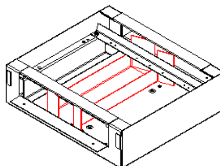
4/3OC* - 4 Compartment Service Box to suit 3 Compartment Trunking *OC = Off Centre
